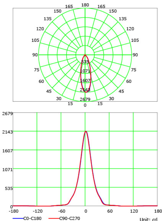
Luminous Intensity Distribution Curve
