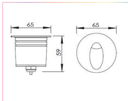
Round Fixture Dimensions
