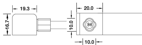
Side Entry Connector MJ-SF16-D5-S02SM MJ-SF16-D5-S03SFM
