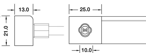
Side Entry Connector MJ-SF15-RGBW-S01/02/03 MJ-SF15-RGBW-S01SM MJ-SF15-RGBW-S02SF MJ-SF15-RGBW-S03SFM
