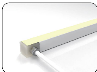
Side Entry Connector MJ-SF16-RGBW-S01/02/03 MJ-SF16-RGBW-S01SM MJ-SF16-RGBW-S02SF MJ-SF16-RGBW-S03SFM
