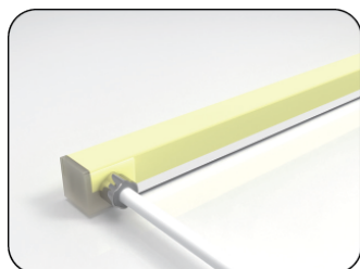
Side Entry Connector MJ-SF18-DW-S01/02/03 MJ-SF18-DW-S01SM MJ-SF18-DW-S02SF MJ-SF18-DW-S03SFM
